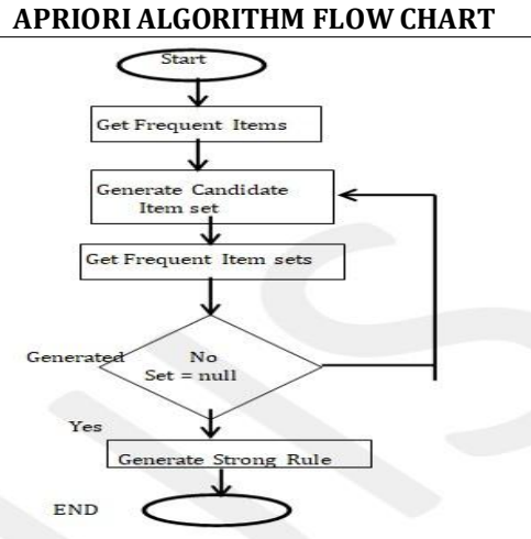
Fig 2: Apriori Flow chart
